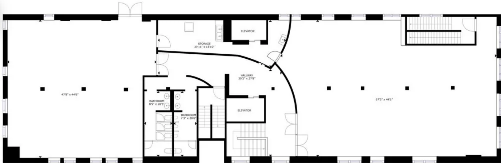
FLOOR 2
