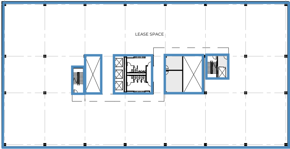
Floor 6
