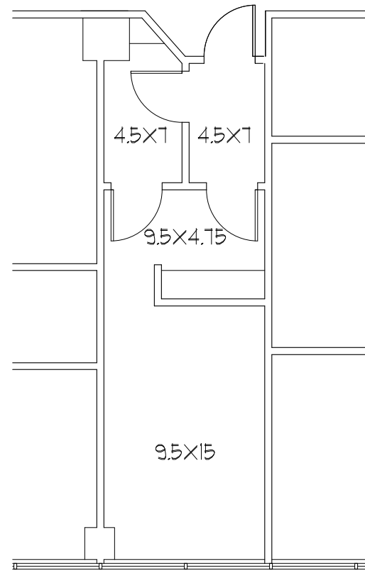
PUBLIC CORRIDOR
