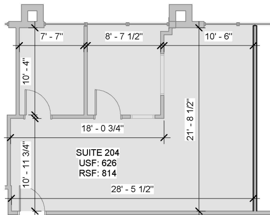
1 SUITE 204 FLOOR PLAN 1/8" = 1'-0"
