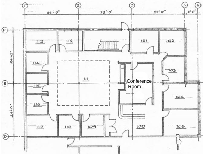
— FIRST FLOOR PLAN (EXISTING CONDITIONS)
