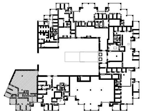
Building Plan
