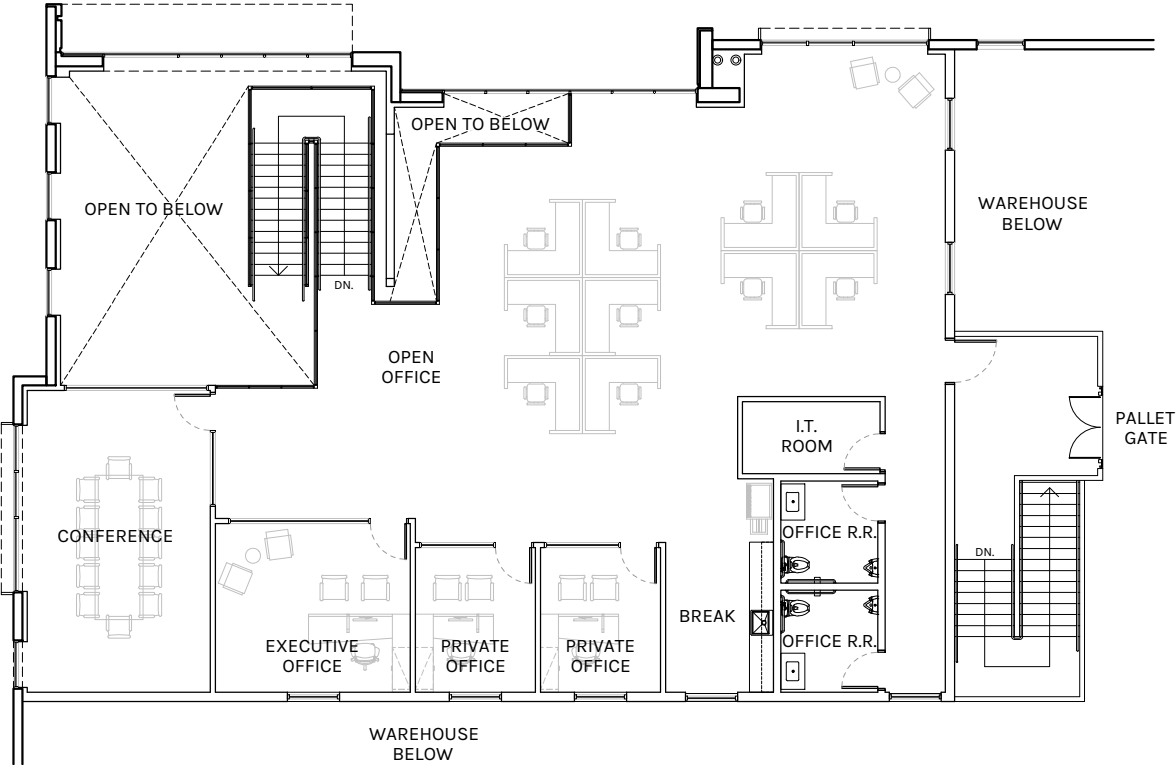
02 MEZZANINE FLOOR PLAN SCALE: AS NOTED
