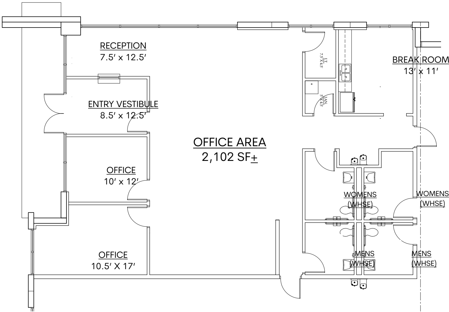
OFFICE PLAN
