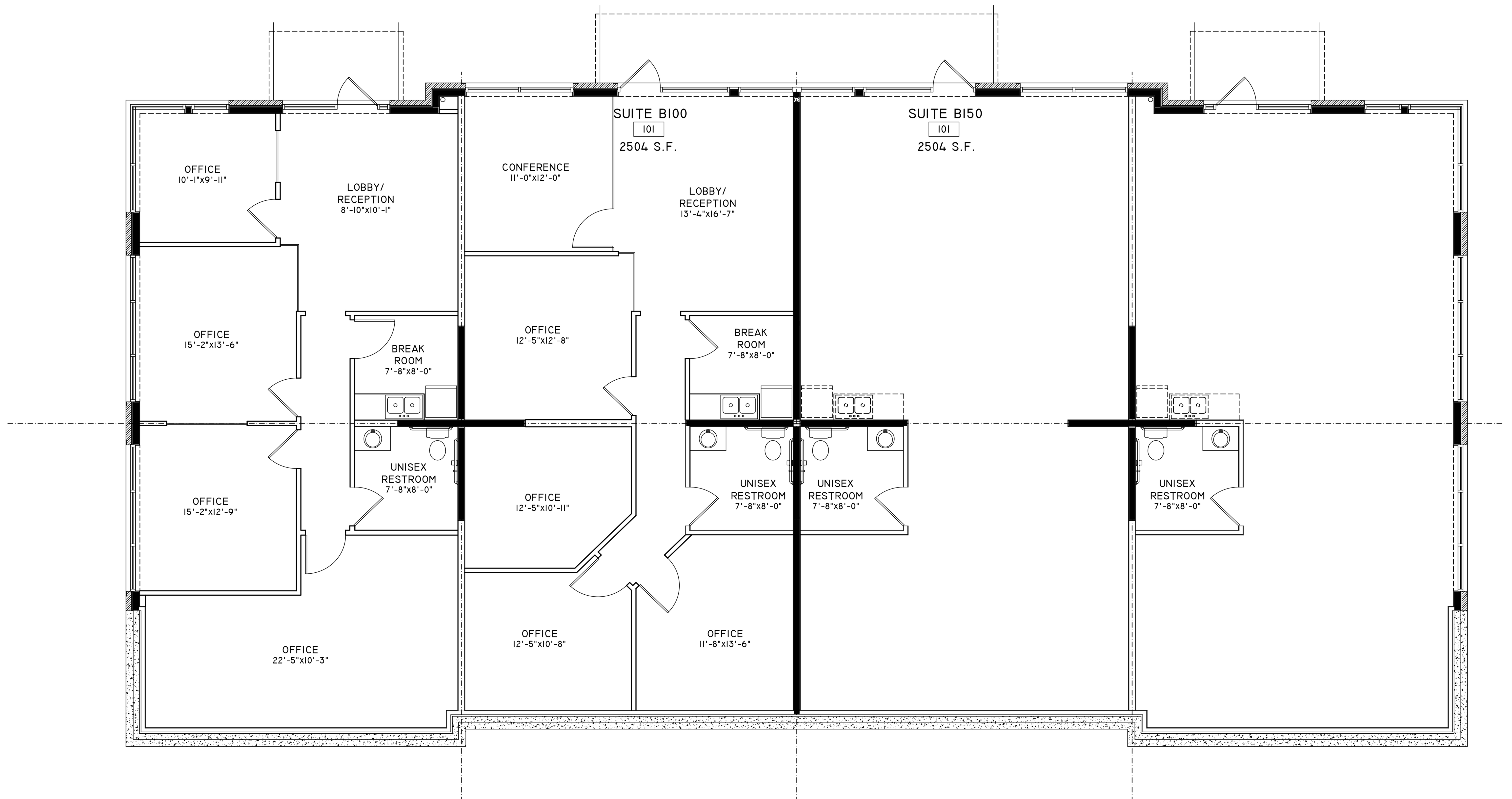
GROUND FLOOR
