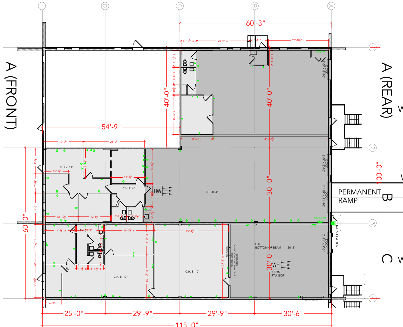
Floor Plan
