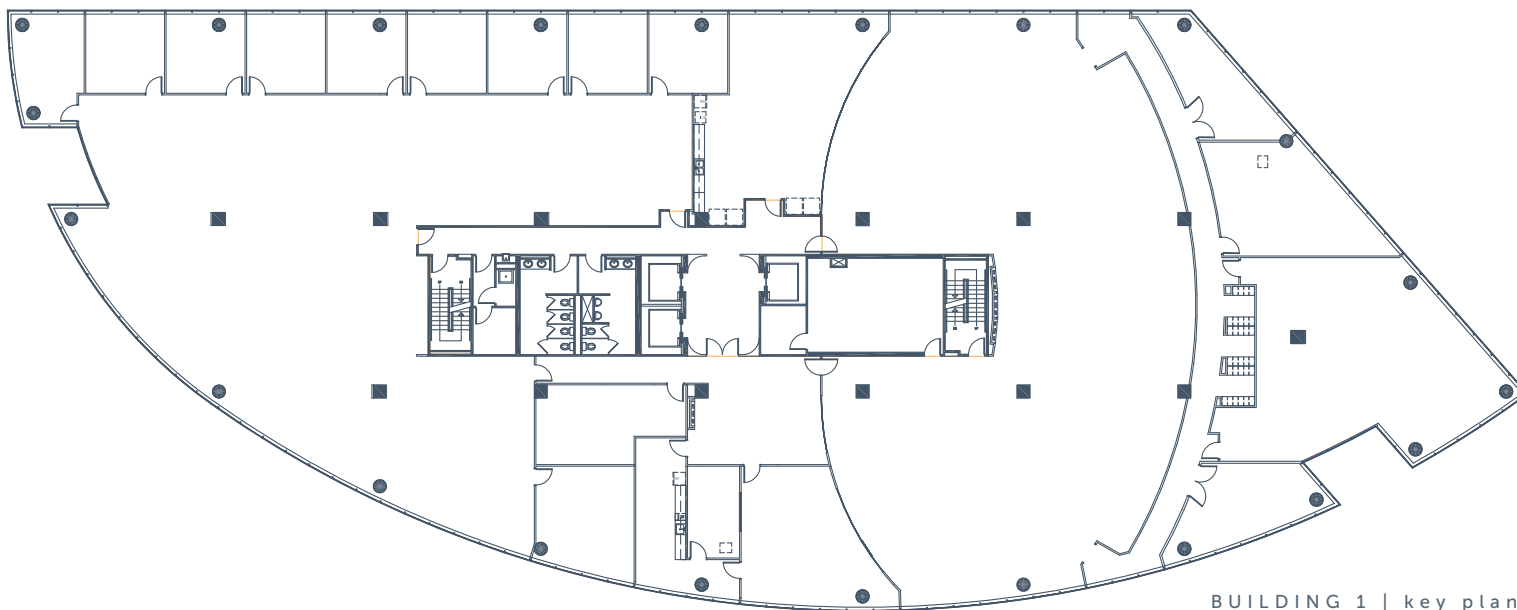
BUILDING 1 | key plan
