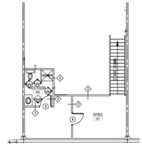
MEZZANINE PLAN
