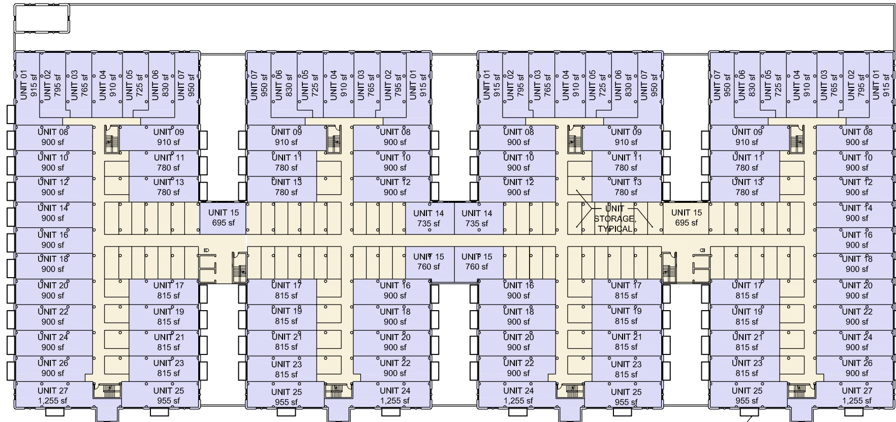
Building A 23,525 sf net per floor 31,640 sf gross per floor 27 units per floor
