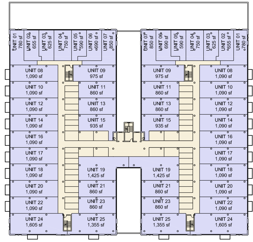
Building E 23,525 sf net per floor 30,685 sf gross per floor 25 units per floor
