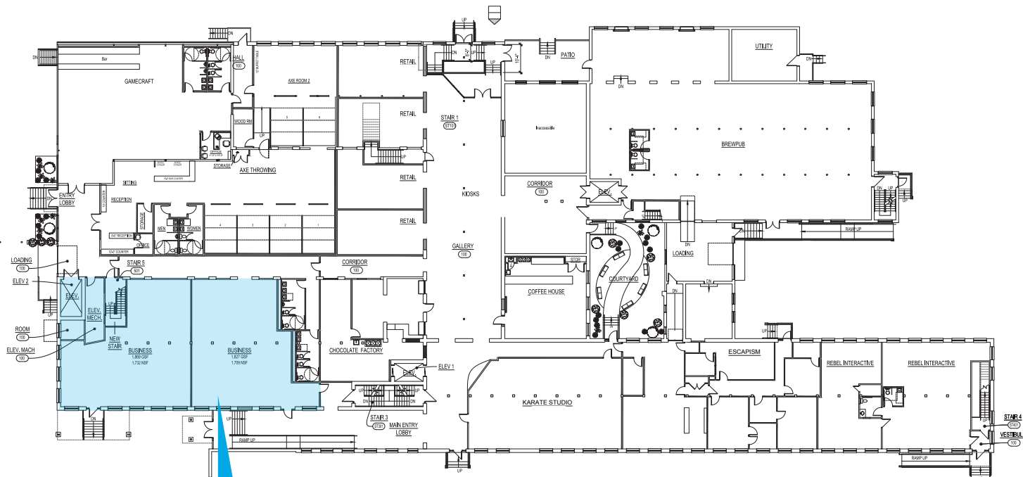
1 FIRST FLOOR CONSTRUCTION PLAN SHEET 101-102
