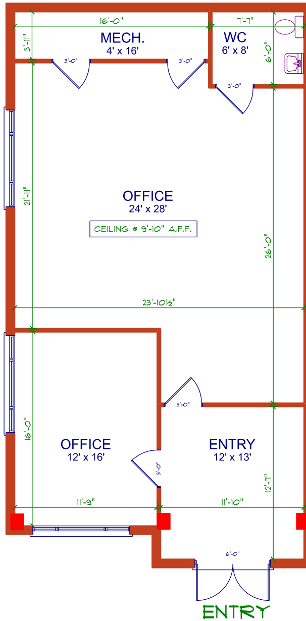
MAIN FLOOR PLAN SUITE 790A - 1138 SF
