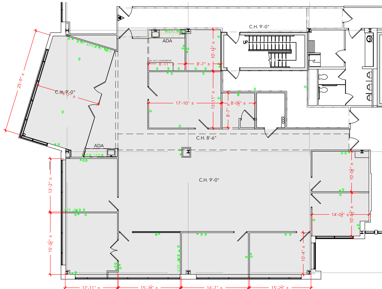
Floor Plan
