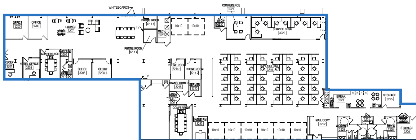
1 SUITE 3260 FLOOR PLAN 1/16" = 1'-0" 0 4 8 16 32 SCALE: 1/16" = 1'-0" NORTH
