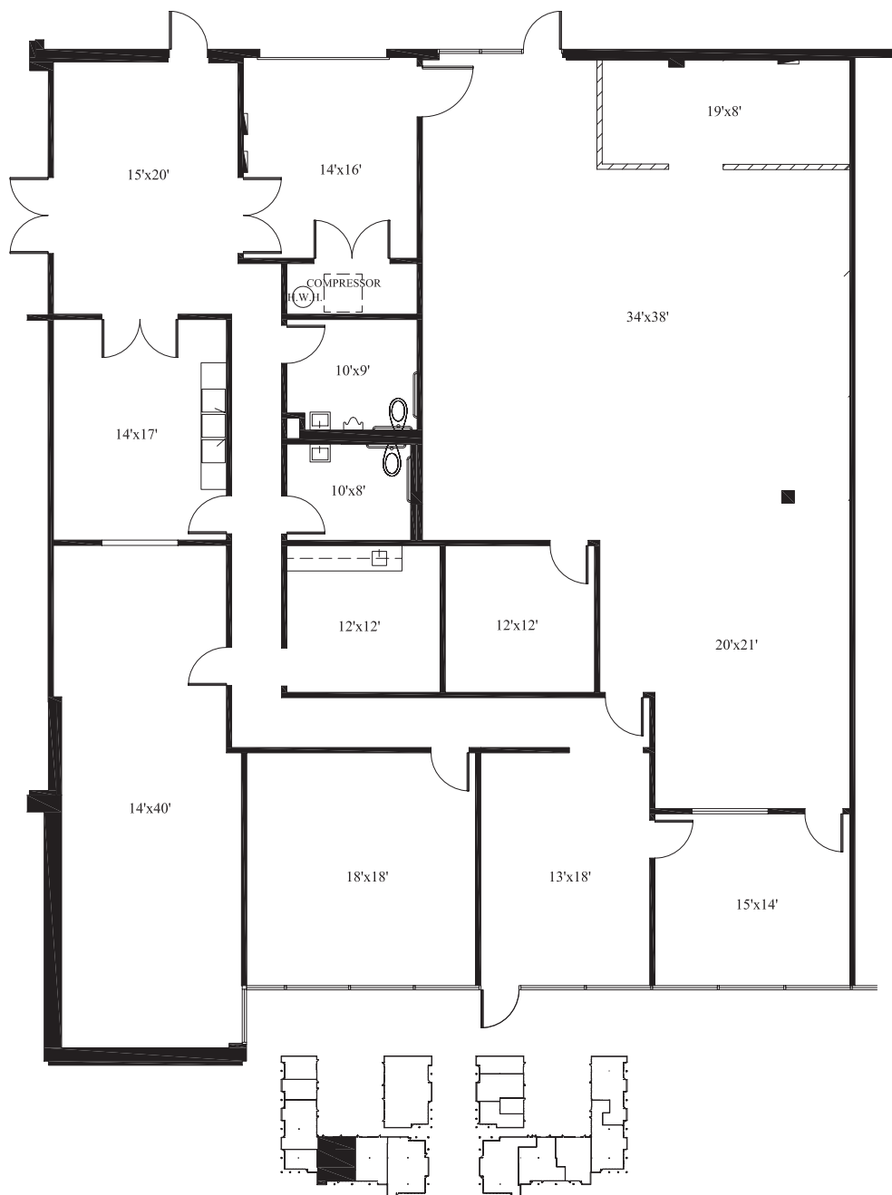
KEY PLAN
