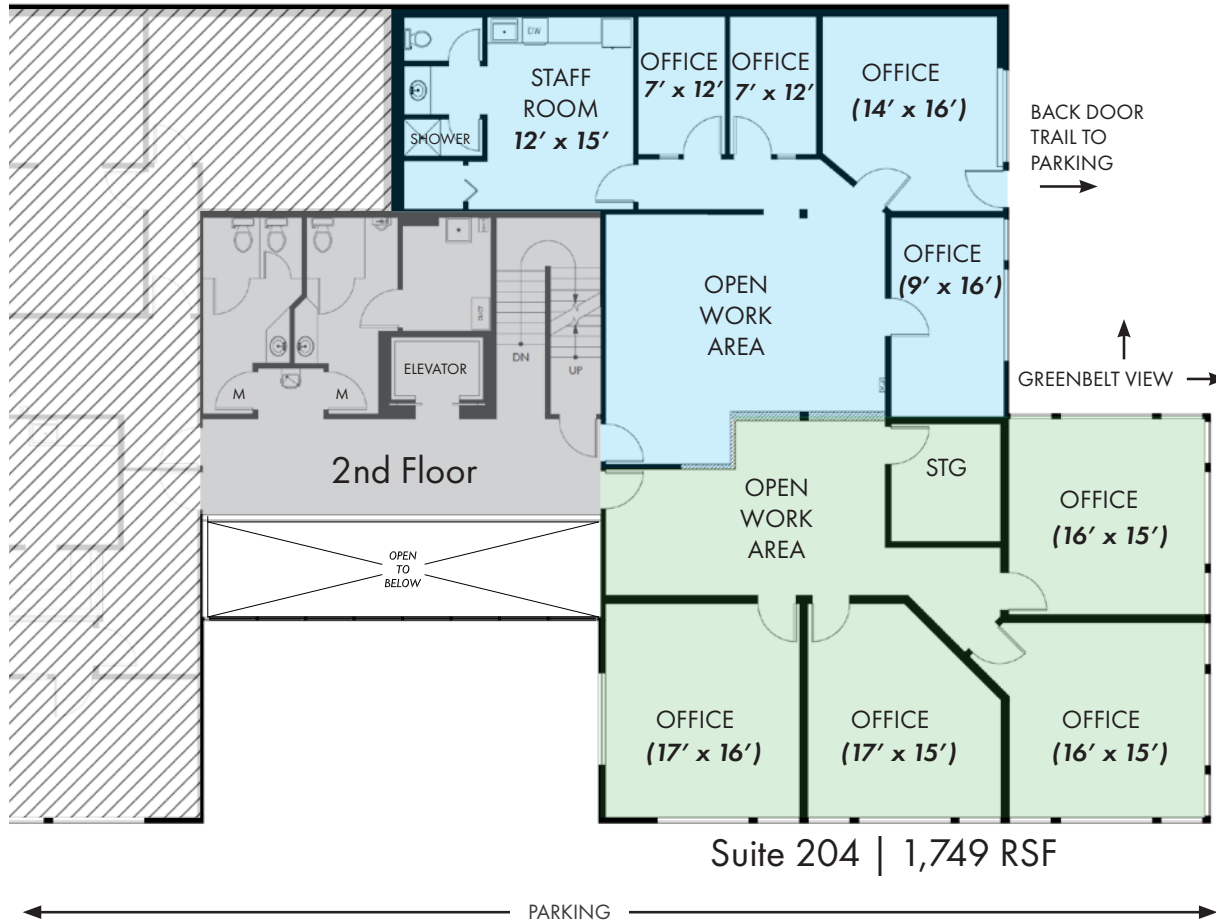
Suite 203 | 1,543 RSF
