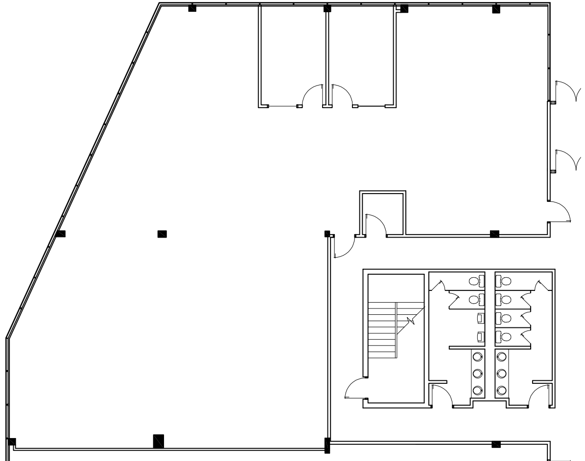
ENLARGED FLOOR PLAN N.T.S.
