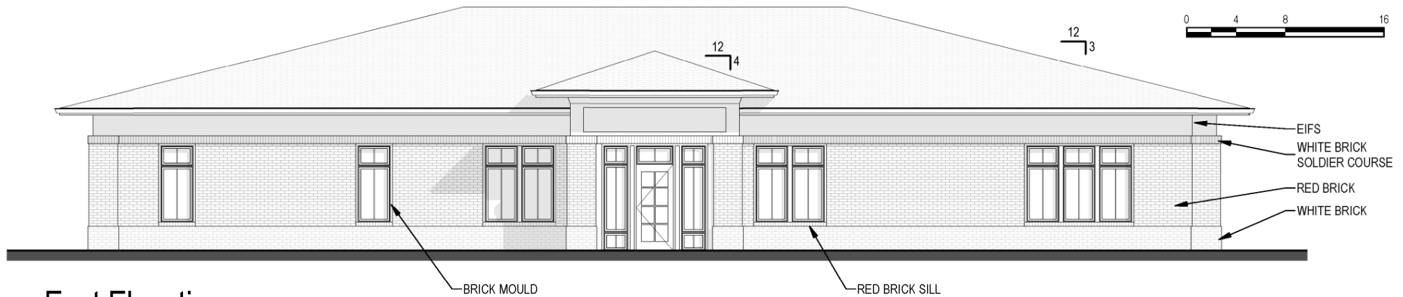
East Elevation
