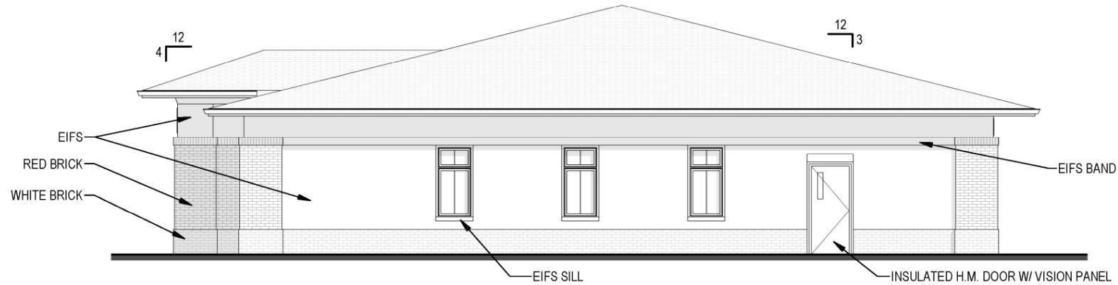
North Elevation
