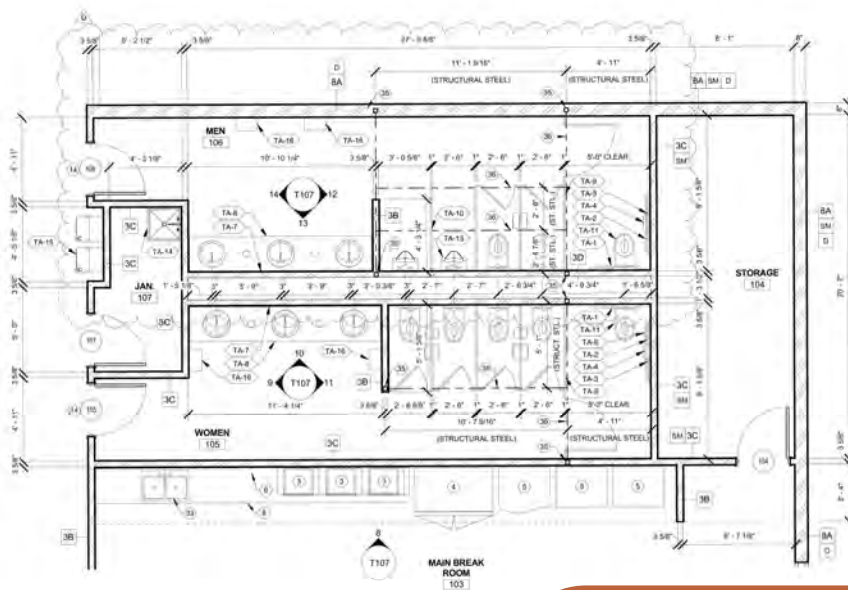
Receiving/Breakroom 1,480 SF
