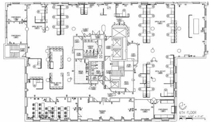
Sixth Floor
