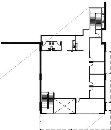
02 MEZZANINE LEVEL PLAN
