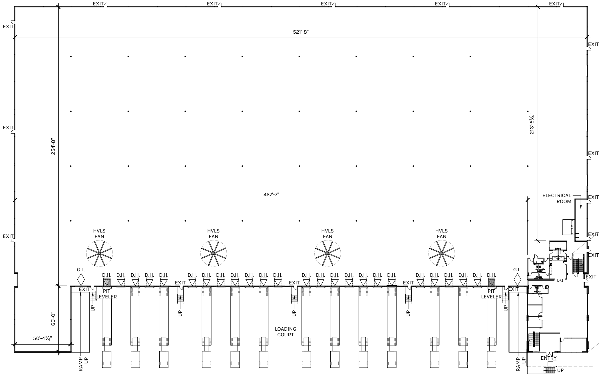
01 GROUND LEVEL PLAN
