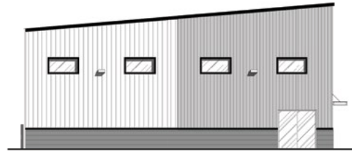
④ BLDG. B WEST ELEVATION 1/8" = 1'-0"
