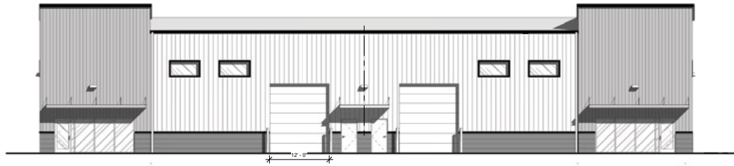
① BLDG. B. SOUTH ELEVATION 1/8" = 1'-0"
