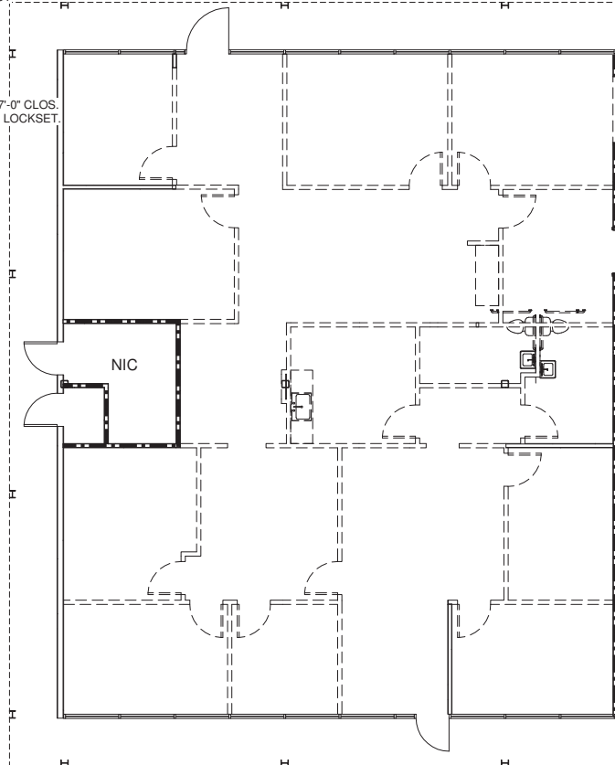
③ Demolition Plan 1/8" = 1'-0"
