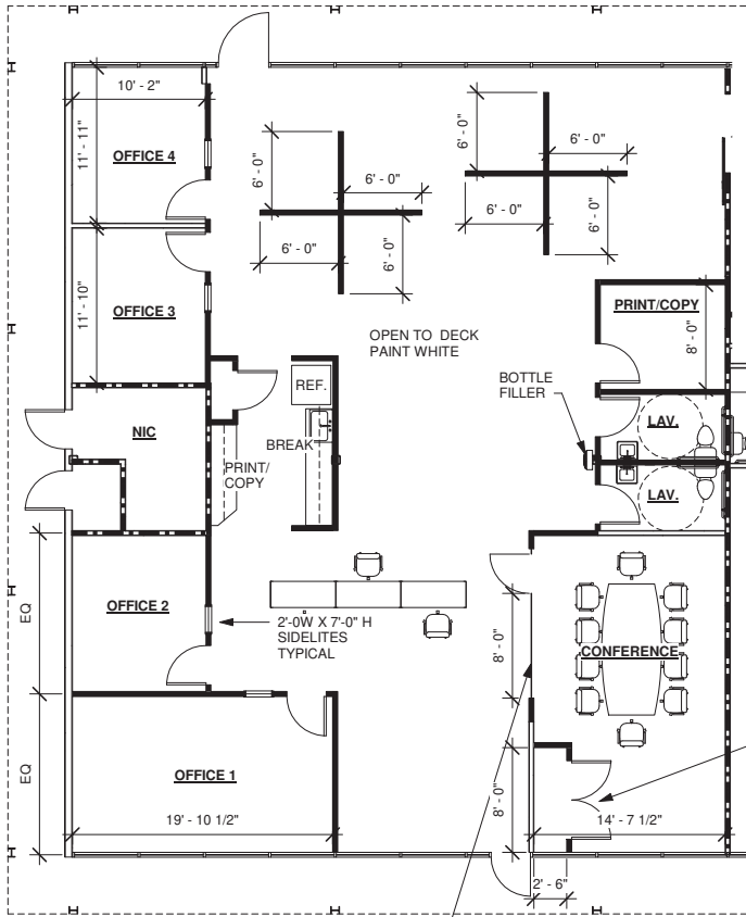
① Preliminary Plan- 4,540 RSF 1/8" = 1'-0"
