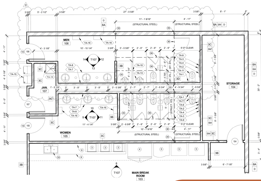
Receiving/Breakroom 1,817 SF
