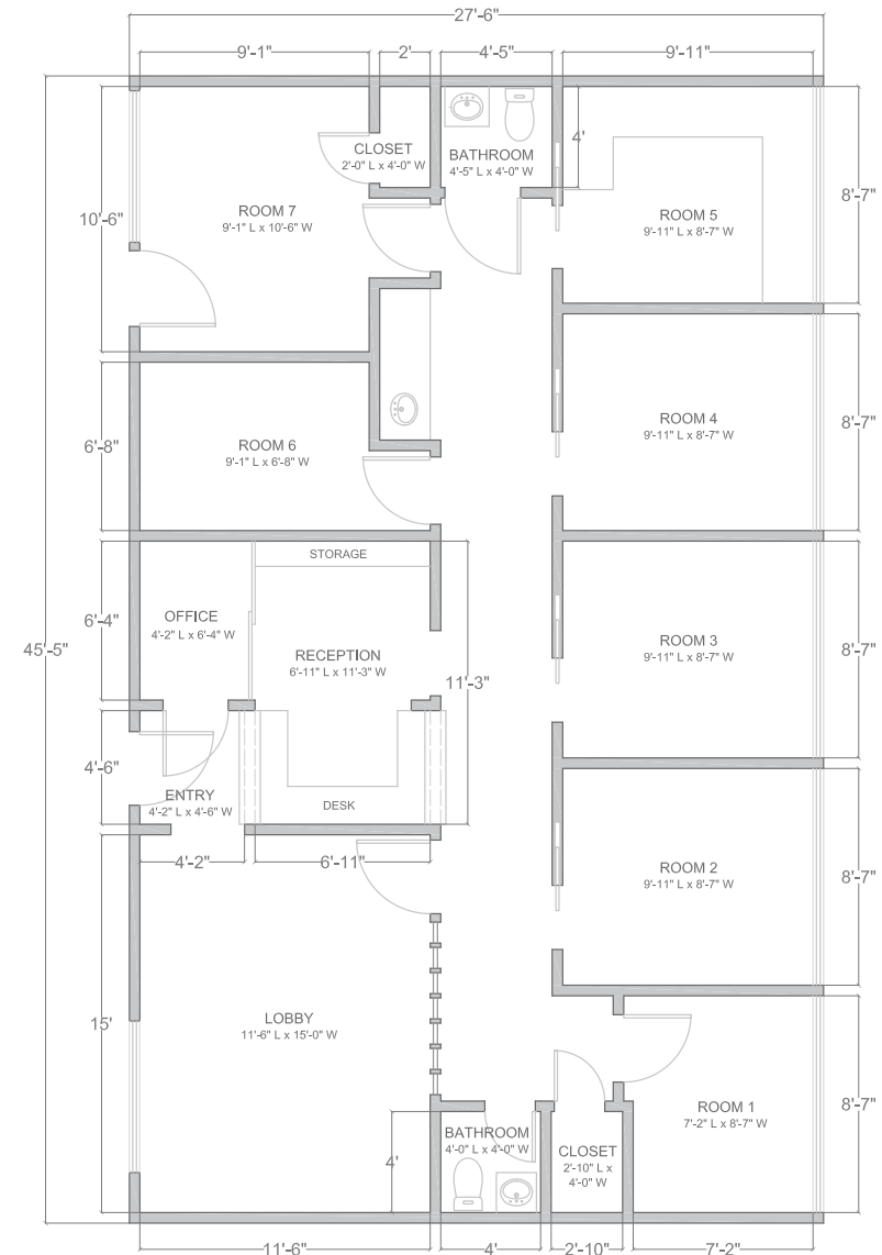
SUITE 206 1,189 SF
