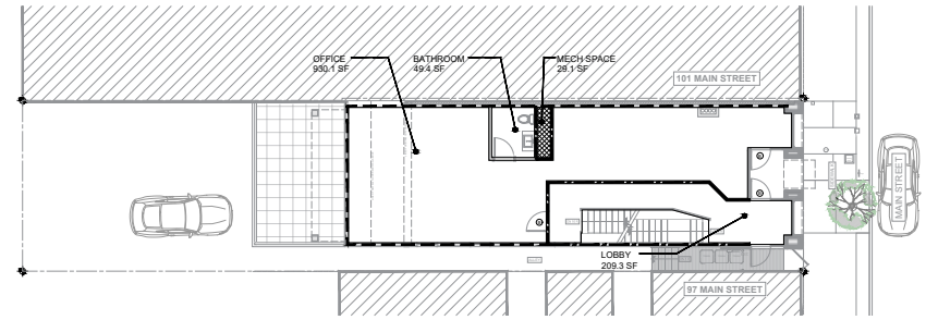
02 FIRST FLOOR OCCUPANCY PLAN
