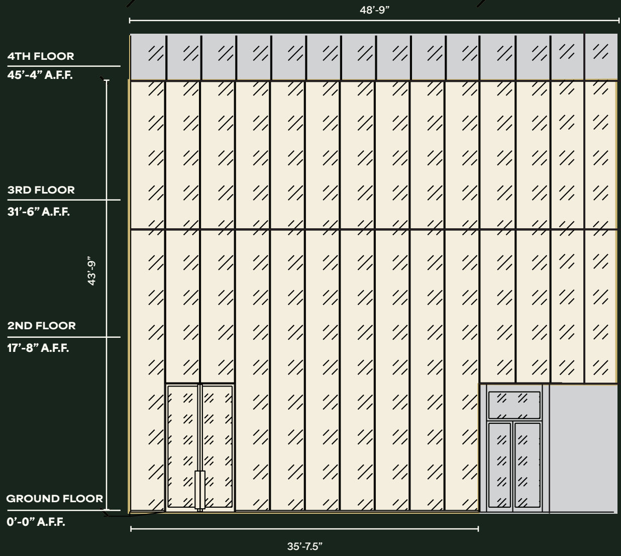
STOREFRONT ELEVATION
