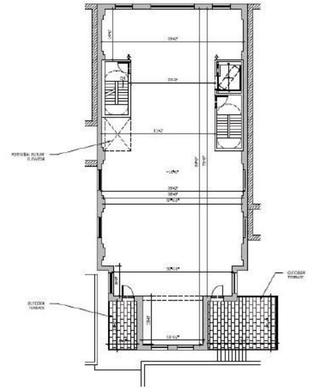
2ND FLOOR PLAN - 3,657 GSF
